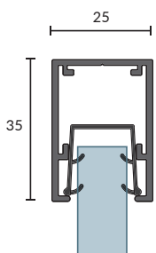
SG25-DEF HEAD CHANNEL / WALL ABUTMENT
