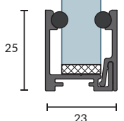
SG25 BASE CHANNEL
