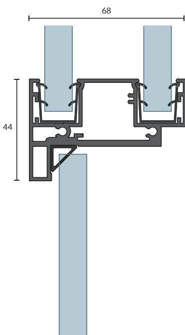
DGF DG FRAME SINGLE LEAF DOOR
