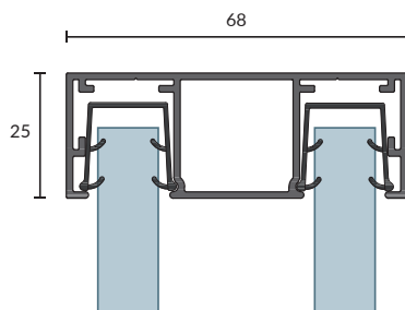
DG68 HEAD CHANNEL / WALL ABUTMENT
