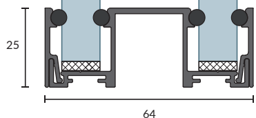
DG68 BASE CHANNEL
